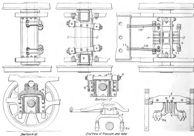
Figs. 3407-3413. Radial Trailing Truck for Atlantic (4-1-2) Locomotive. Pennsylvania Railroad.
